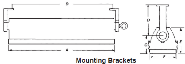
Mounting Brackets
