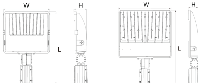
MONTAGE SLIPFITTER
