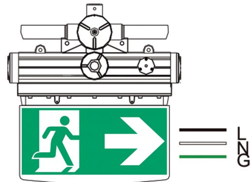
Wall Mounting - Feed through with existing pipes on wall
