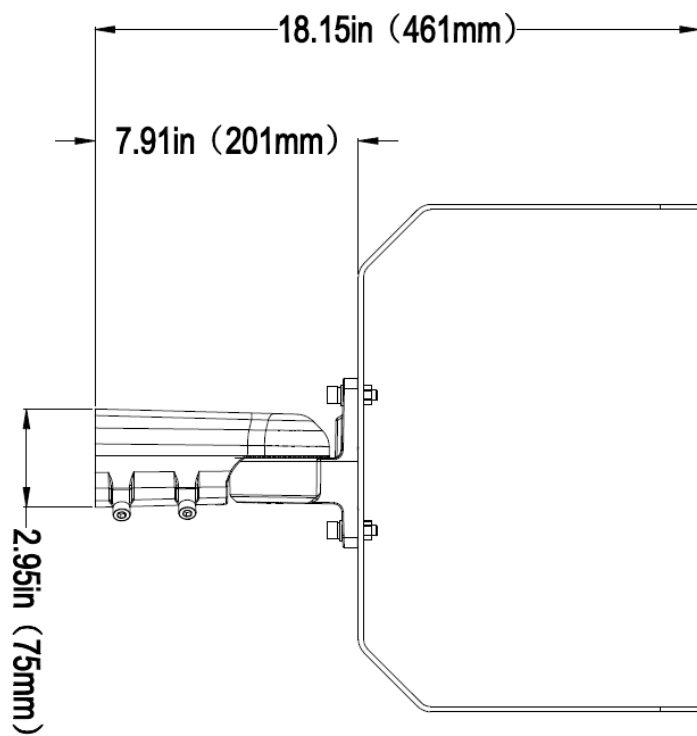
SFU BRACKET
