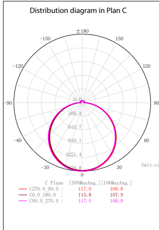
24X24PO,40W
