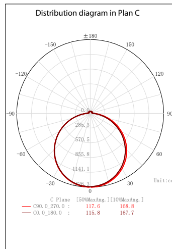
12X48PO,40W
