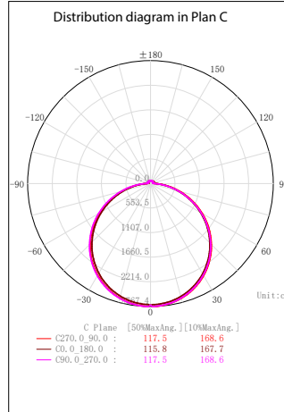
24X48PO,72W
